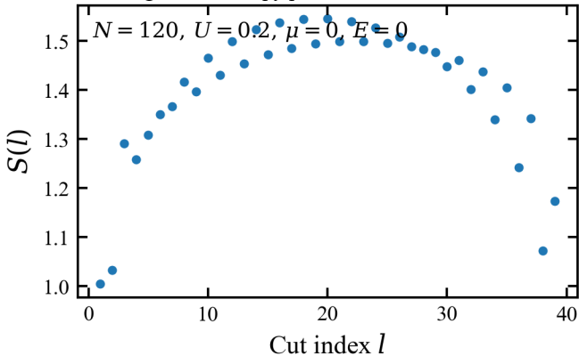
Entanglement entropy profile in the Lieb-Kitaev chain
