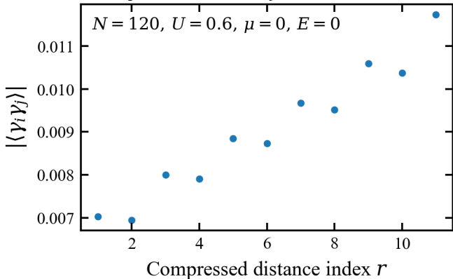
Representative bulk Majorana correlation slice
