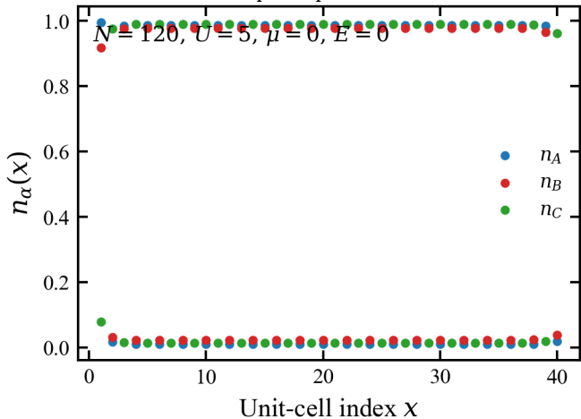
Orbital-resolved occupation profile in the Lieb-Kitaev chain
