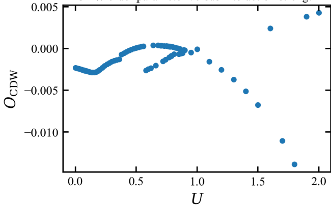
CDW order parameter versus interaction strength
