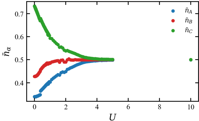
Bulk-averaged orbital occupation versus interaction strength
