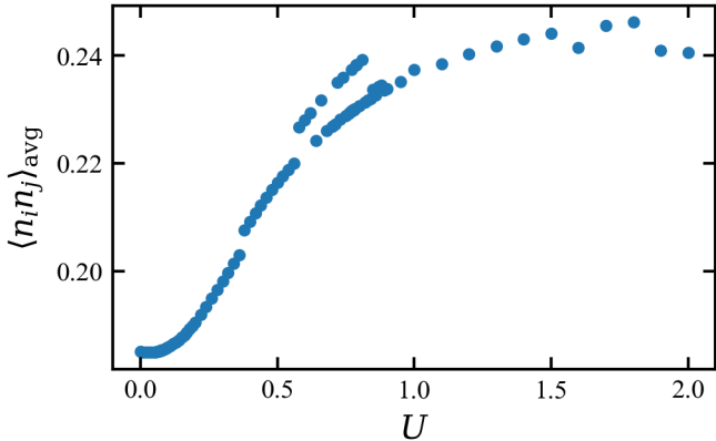
Average density-density correlation versus interaction strength
