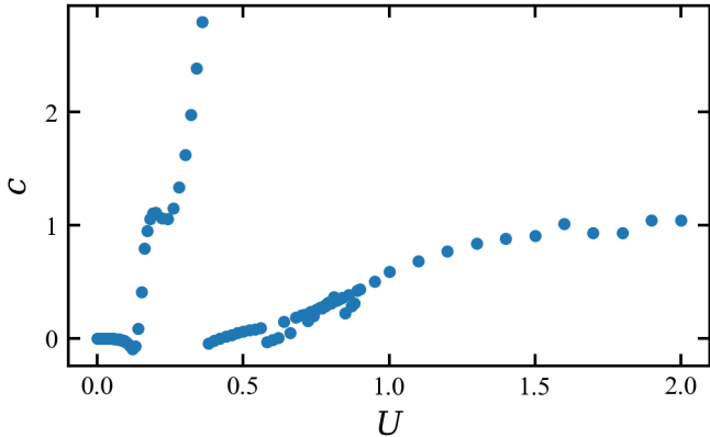
Central charge versus interaction strength
