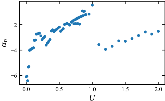
Density-correlation power-law exponent versus interaction strength
