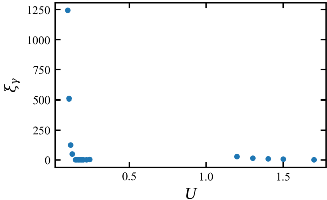
Bulk Majorana correlation length versus interaction strength
