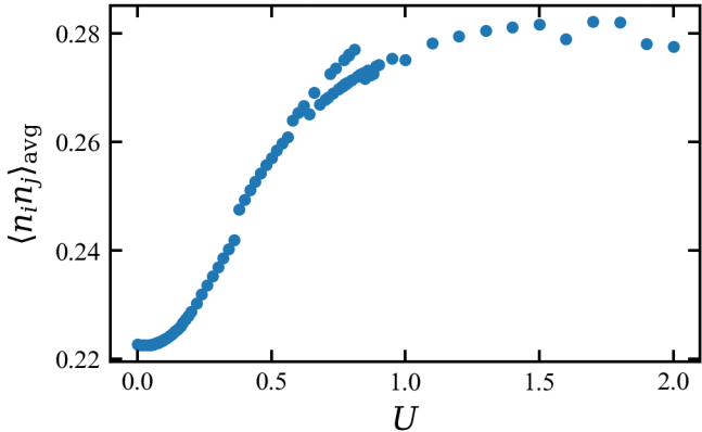
Average orbital density matrix versus interaction strength: nBB
