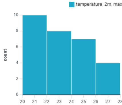
weather_data_histogram_Sydney
