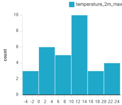
weather_data_histogram_Moscow
