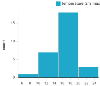
weather_data_histogram_London
