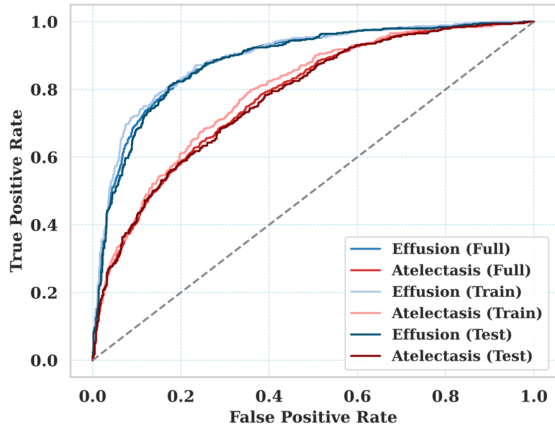
ROC Curve
