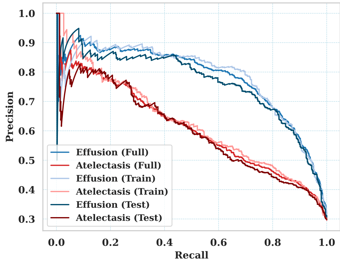
Precision-Recall Curve
