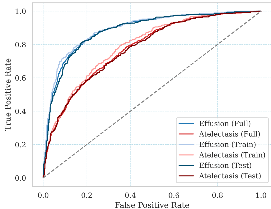
ROC Curve
