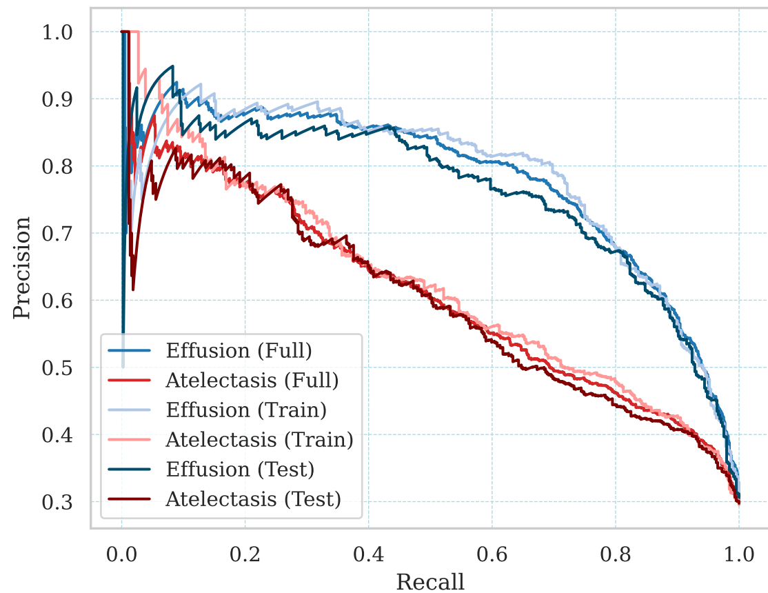
Precision-Recall Curve
