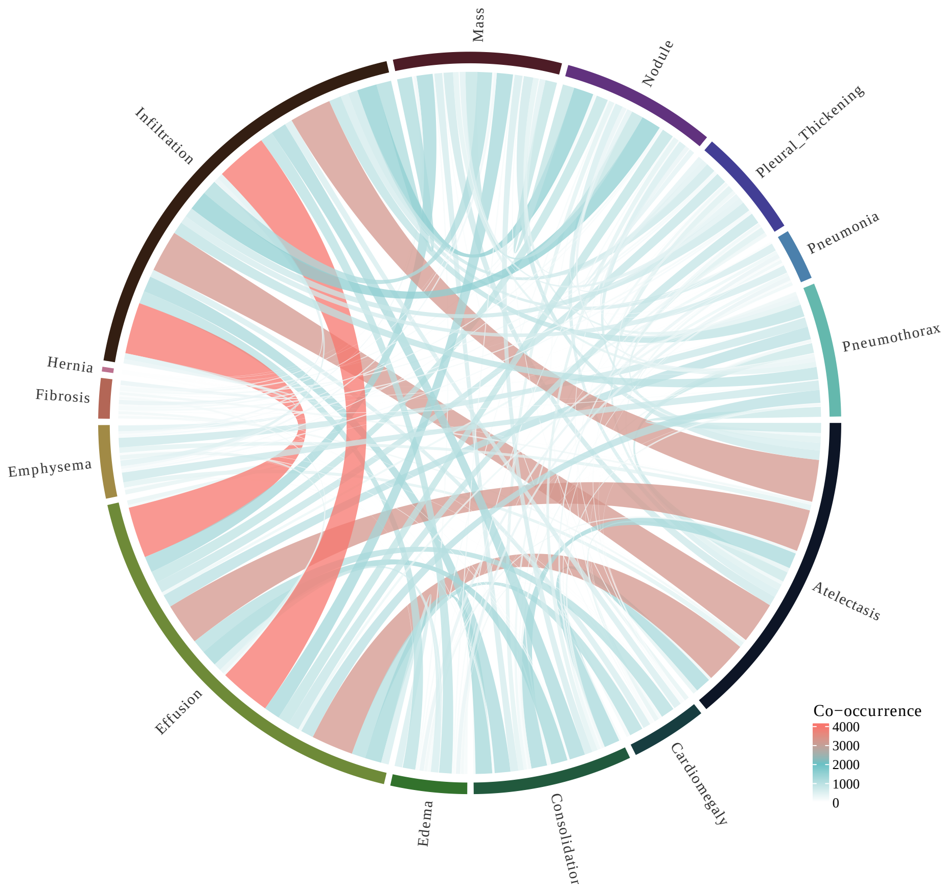
Disease Co-occurrence Chord Diagram
