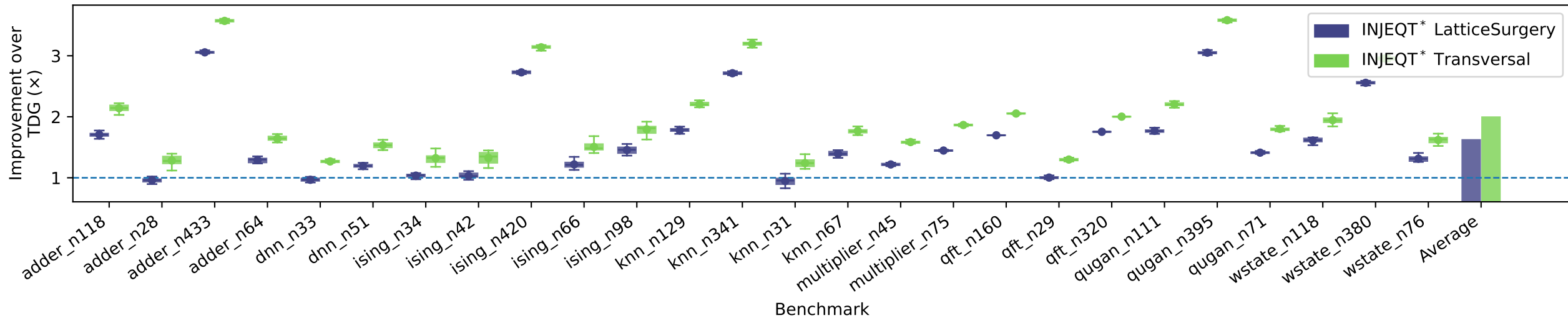
Space-Time: Improvement over TDG (x) (Distillation)
