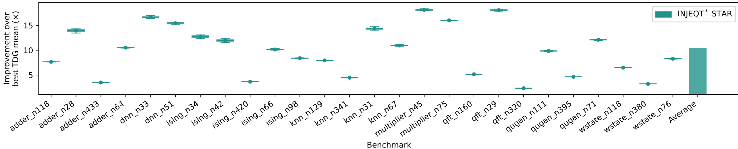
Total Error: Improvement over best TDG mean (x) (STAR)
