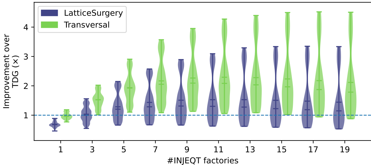
Space-Time: INJEQT sweep over num_factories (Cultivation)
