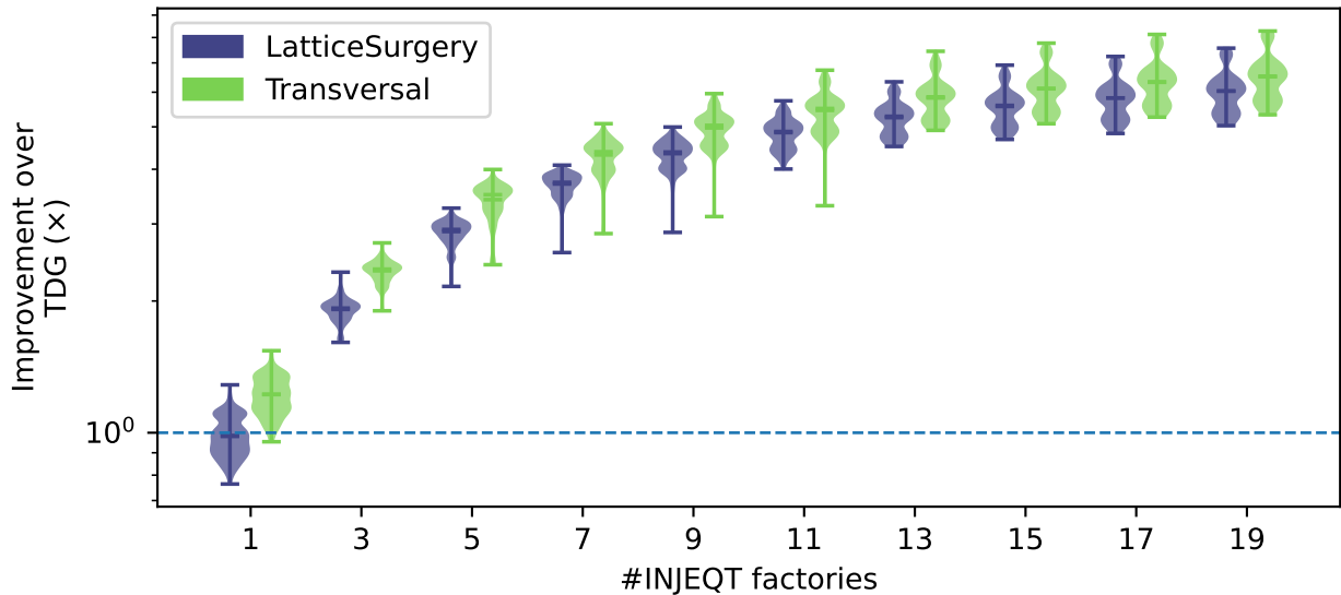
Wall-Clock Time: INJEQT sweep over num_factories (Distillation)
