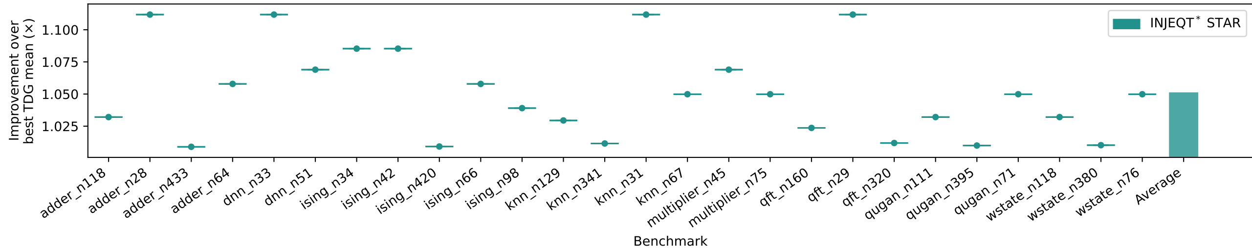
#Physical Qubits: Improvement over best TDG mean (x) (STAR)
