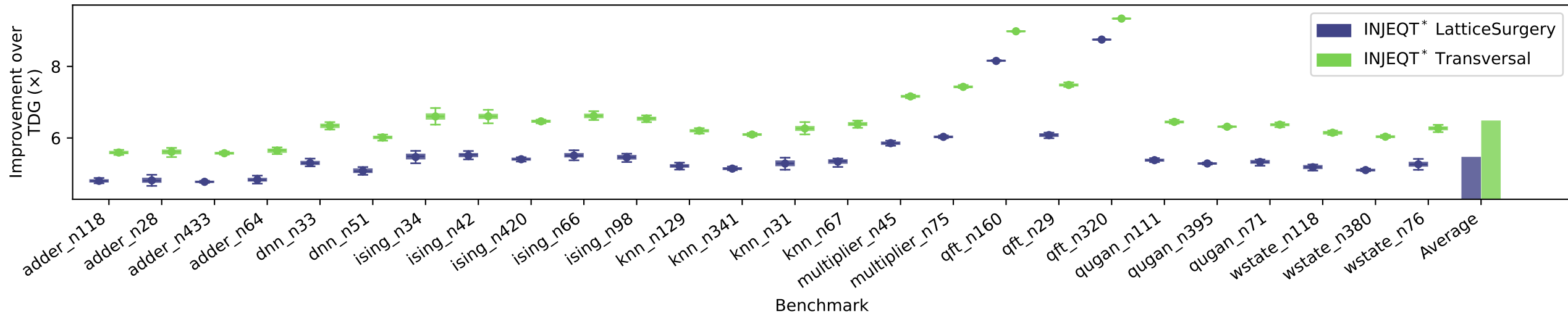
Wall-Clock Time: Improvement over TDG (x) (Cultivation)
