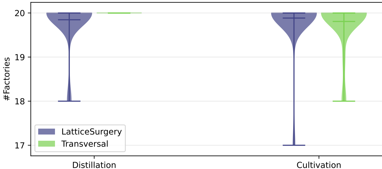
Wall-Clock Time: Optimal INJEQT* factories across benchmarks
