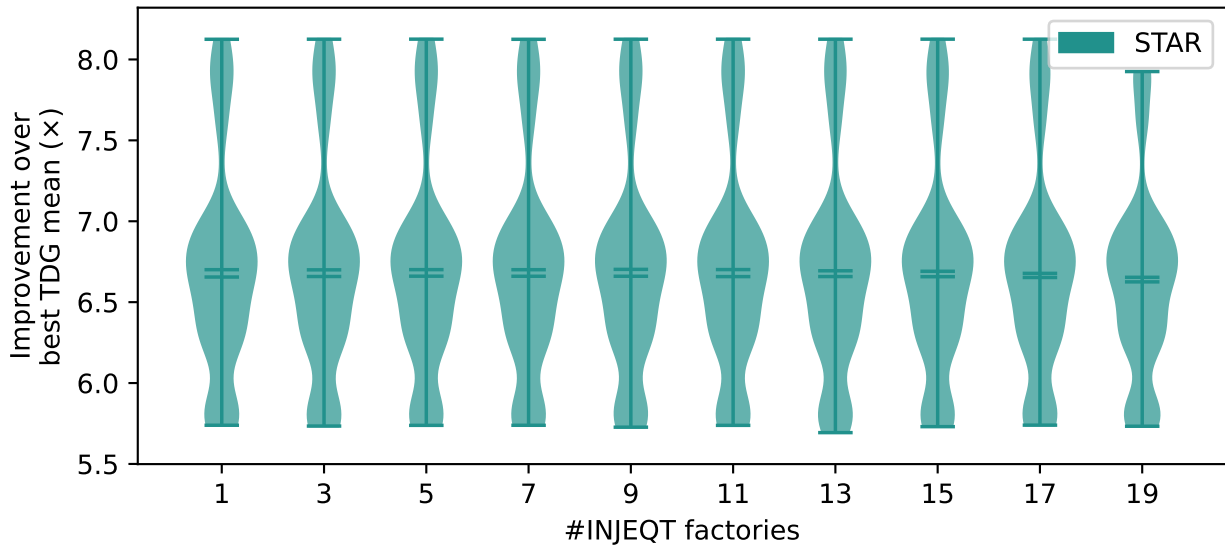
Active Time: INJEQT sweep over num_factories (STAR)
