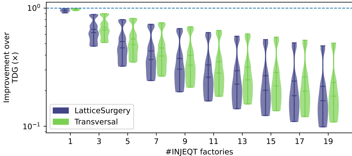
#Physical Qubits: INJEQT sweep over num_factories (Distillation)
