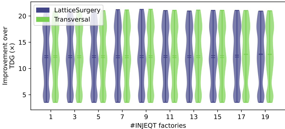
Total Error: INJEQT sweep over num_factories (Cultivation)
