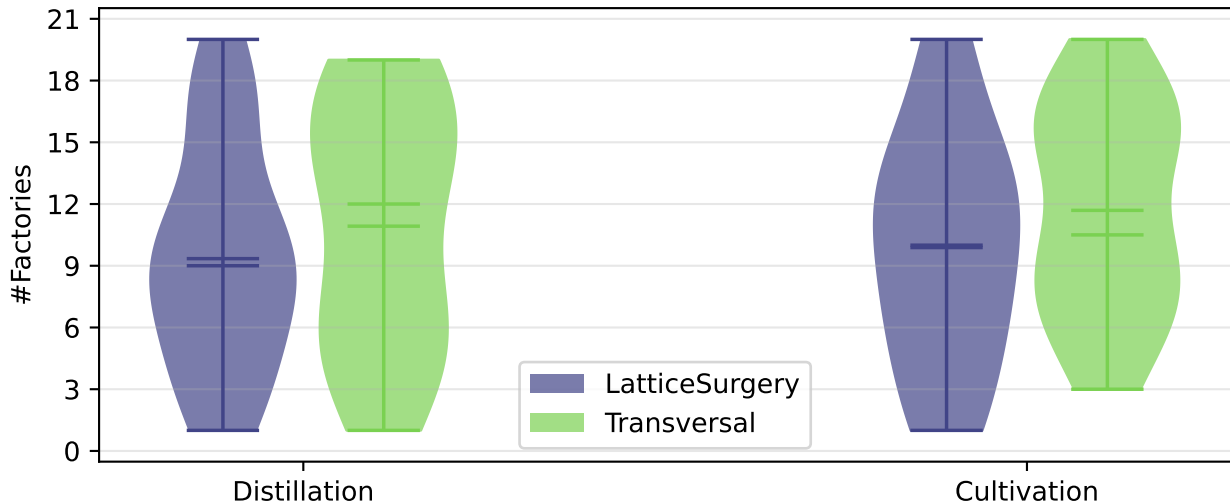
Total Error: Selected INJEQT* num_factories across benchmarks
