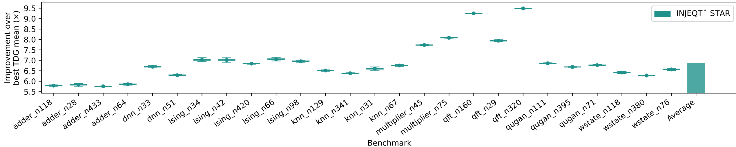
Wall-Clock Time: Improvement over best TDG mean (x) (STAR)
