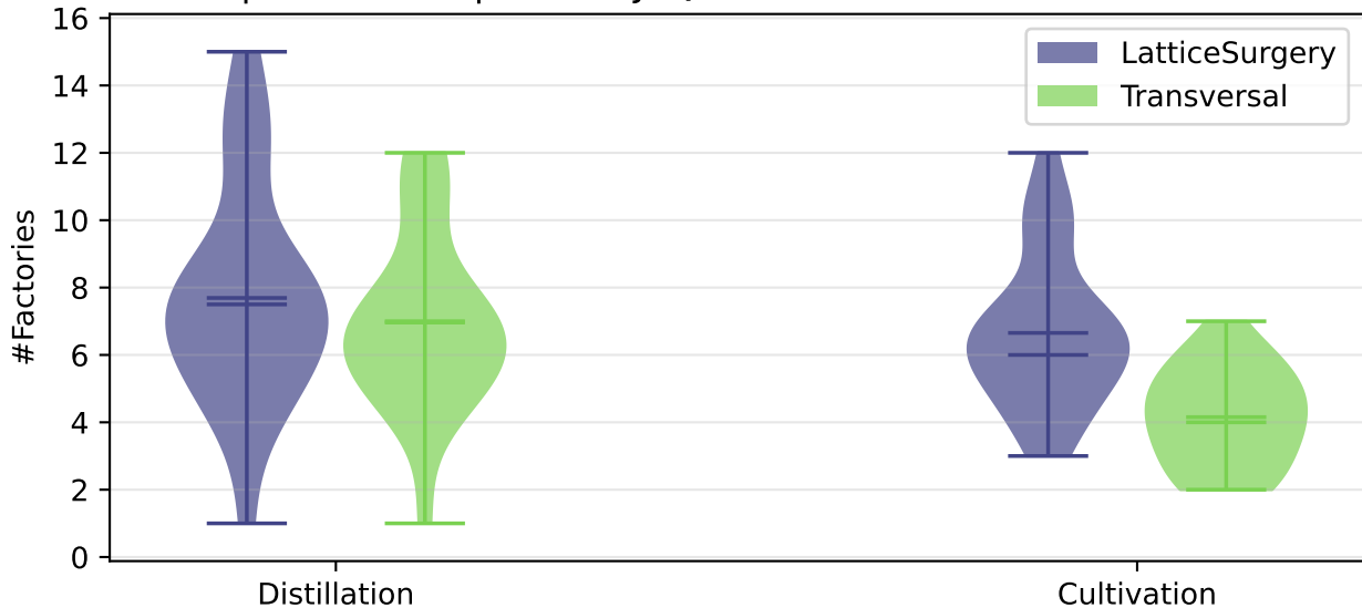
Space-Time: Optimal INJEQT* factories across benchmarks
