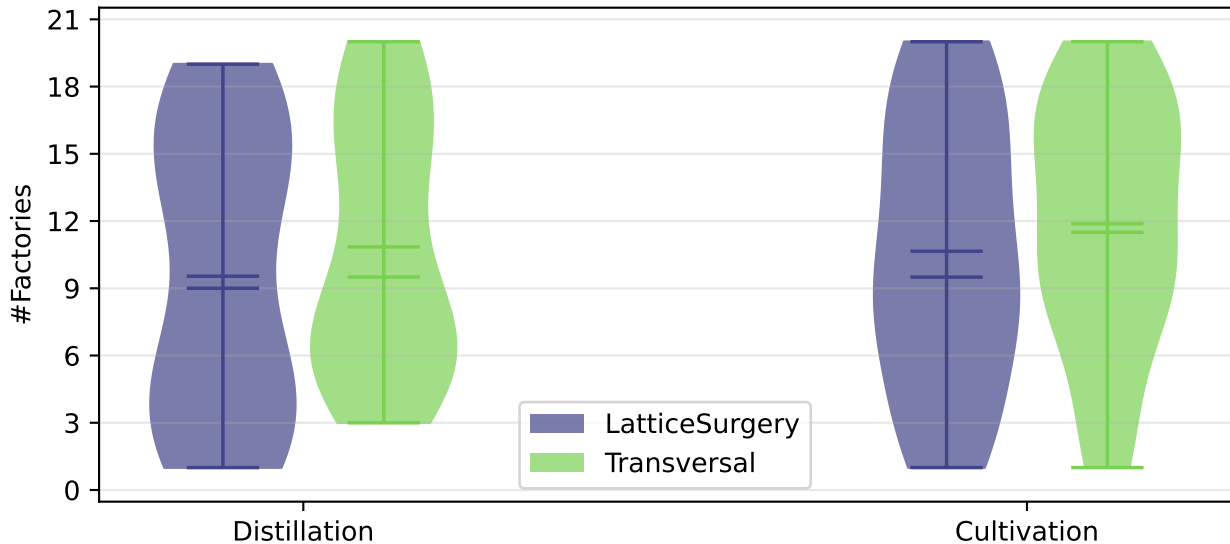
Total Error: Optimal INJEQT* factories across benchmarks
