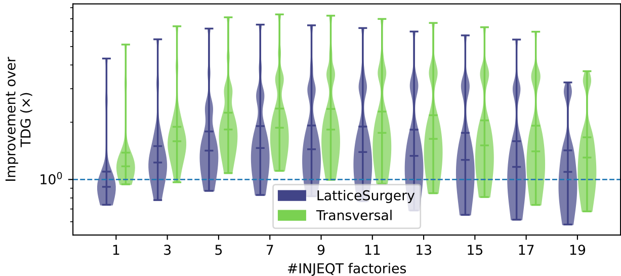
Space-Time: INJEQT sweep over num_factories (Distillation)
