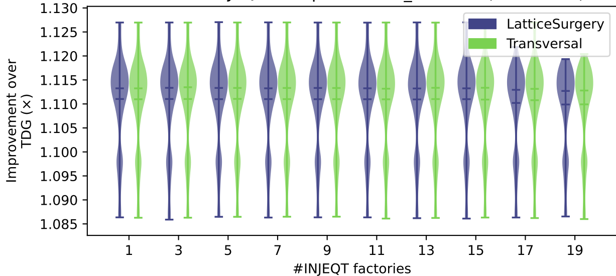
Total Error: INJEQT sweep over num_factories (Distillation)
