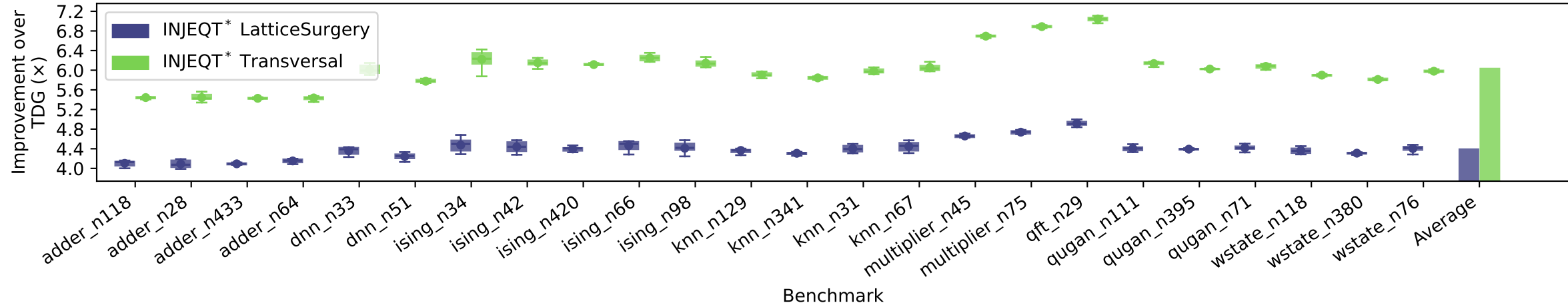
Wall-Clock Time: Improvement over TDG (x) (Cultivation)
