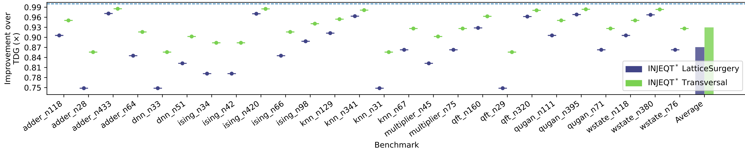
#Physical Qubits: Improvement over TDG (x) (Cultivation)
