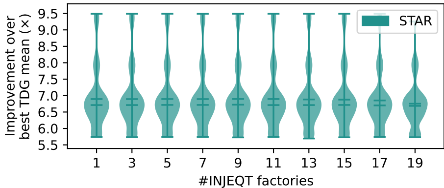
Wall-Clock Time: INJEQT sweep over num_factories (STAR)
