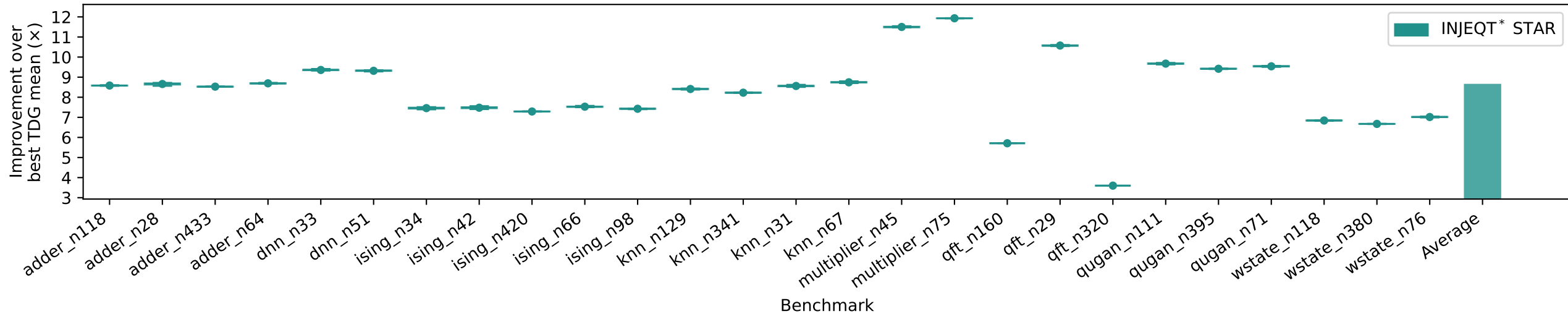
Active Time: Improvement over best TDG mean ( \times ) (STAR)
