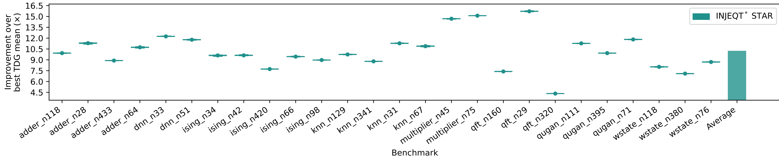
Space-Time: Improvement over best TDG mean (x) (STAR)
