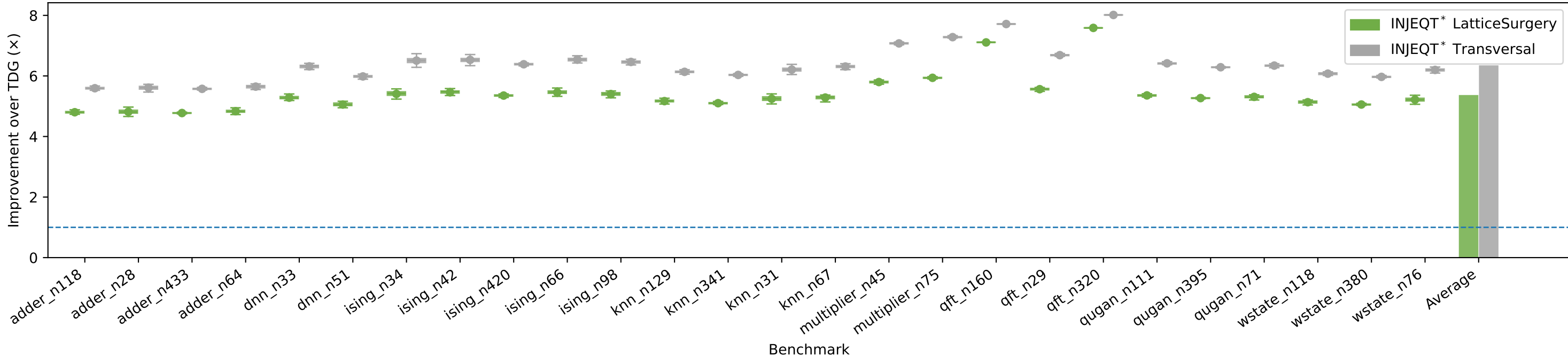
active_time: Improvement over TDG (x) (Cultivation)
