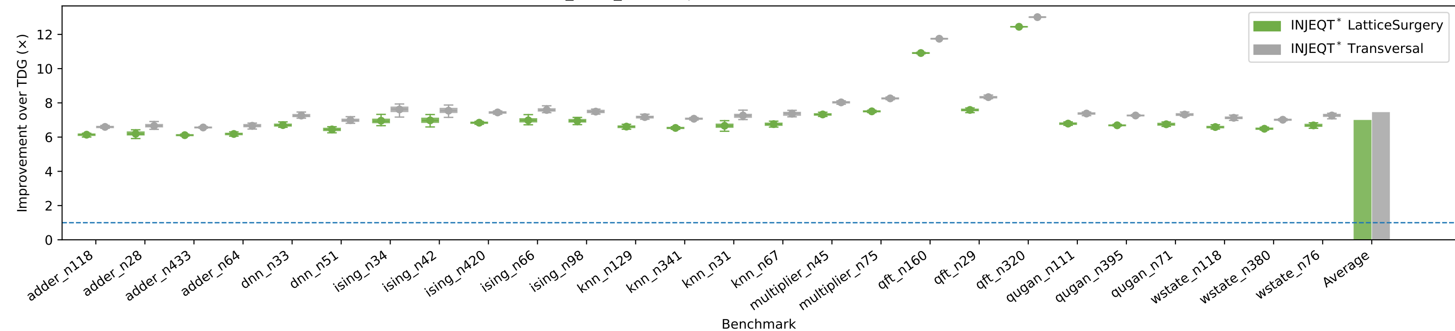
wall_clock_time: Improvement over TDG (x) (Distillation)
