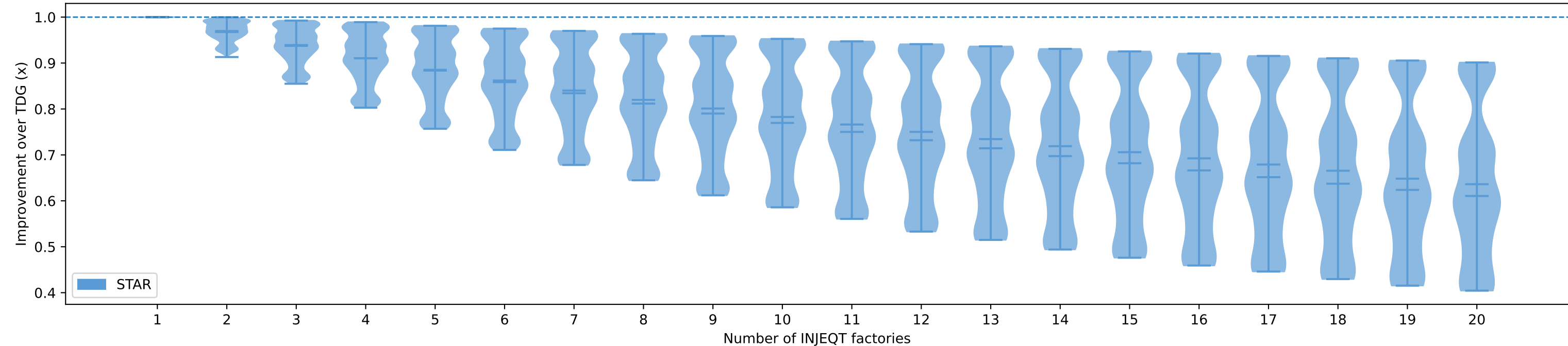
space_time: INJEQT sweep over num_factories (STAR)
