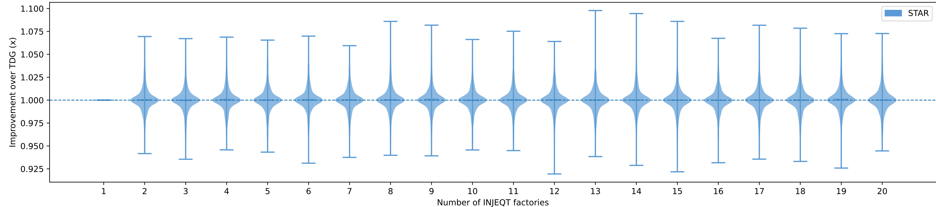
total_error: INJEQT sweep over num_factories (STAR)
