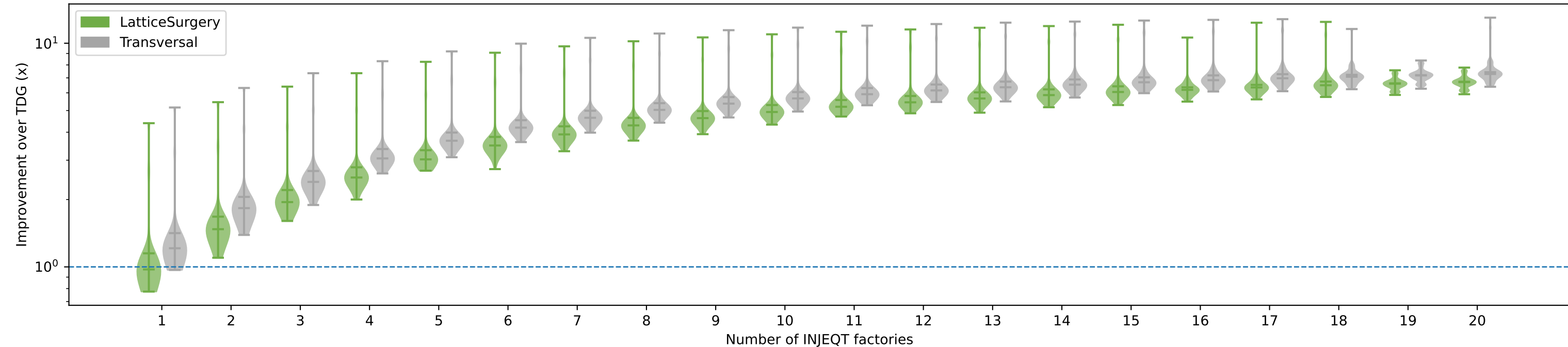
wall_clock_time: INJEQT sweep over num_factories (Distillation)
