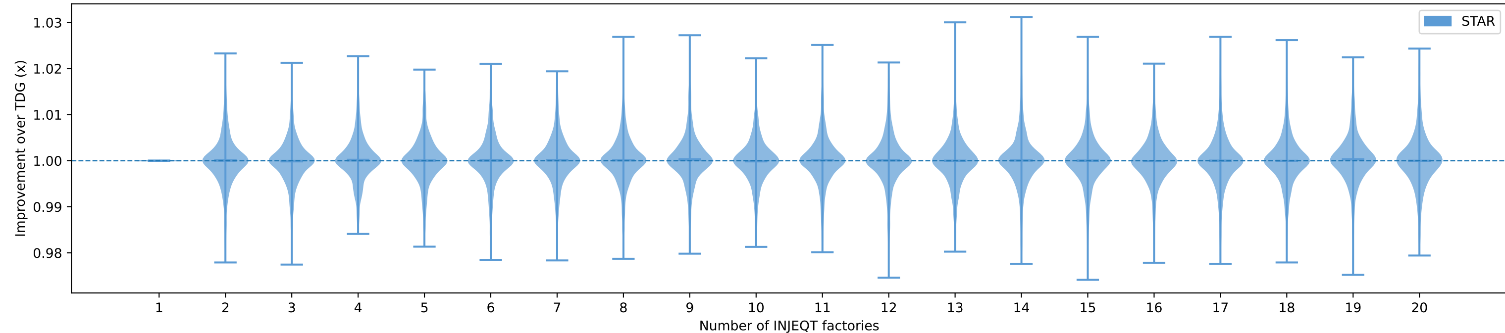
wall_clock_time: INJEQT sweep over num_factories (STAR)
