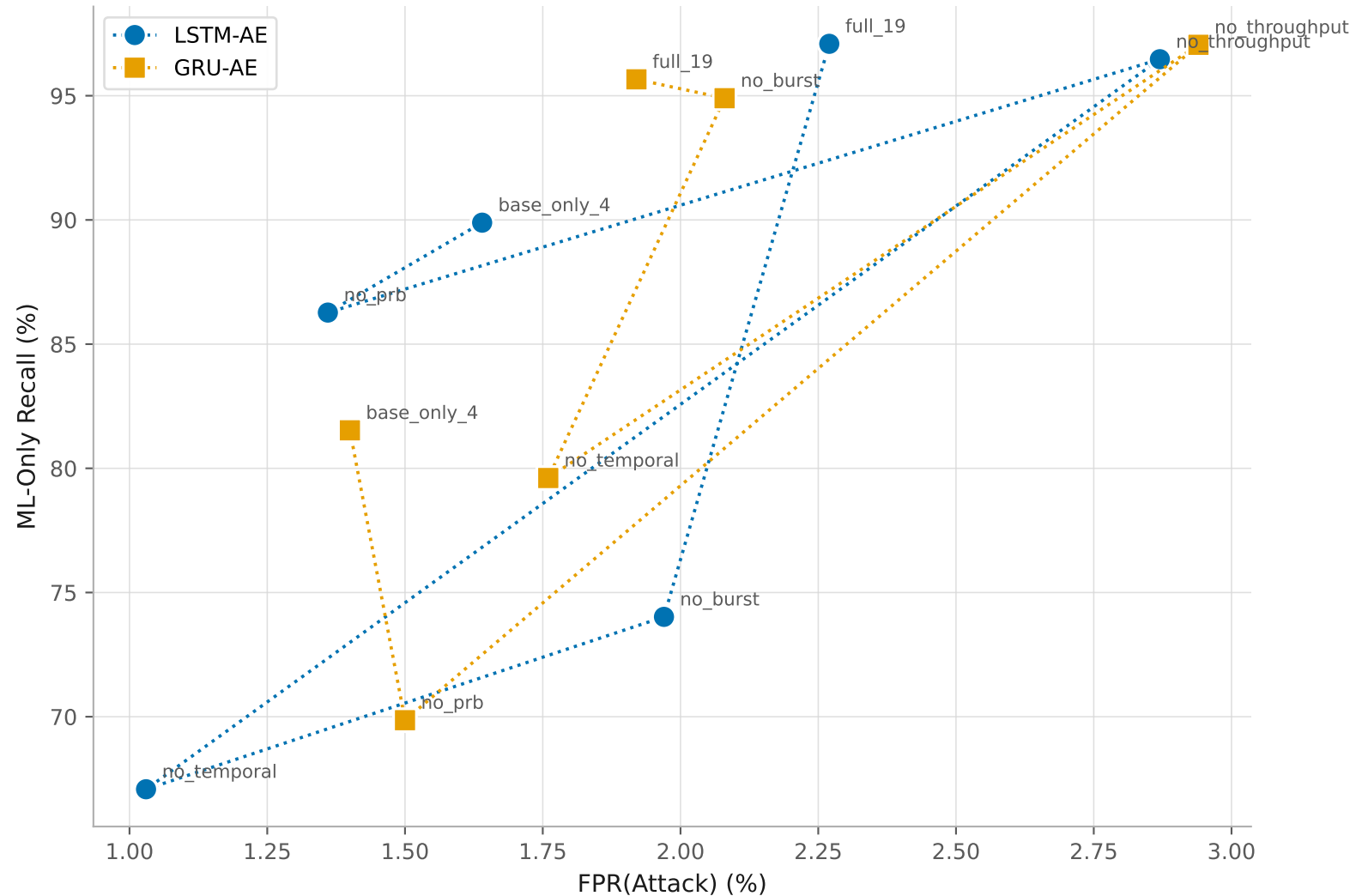
Trade-off FPR(Attack) vs Recall antar Konfigurasi Fitur ML-Only, seed 42
