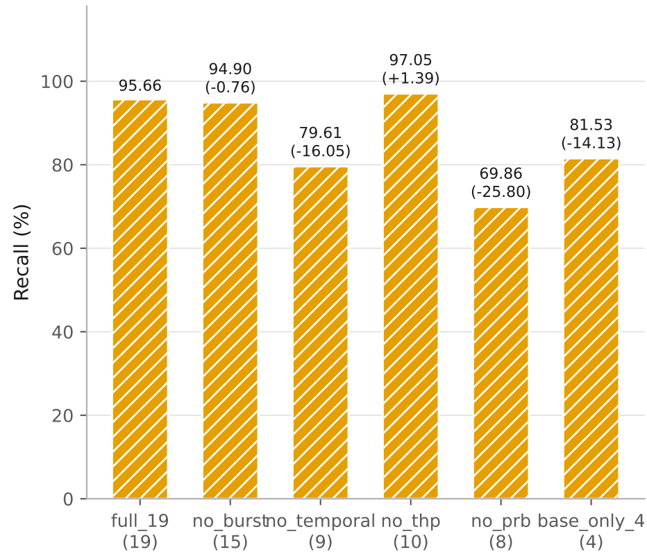
Recall
