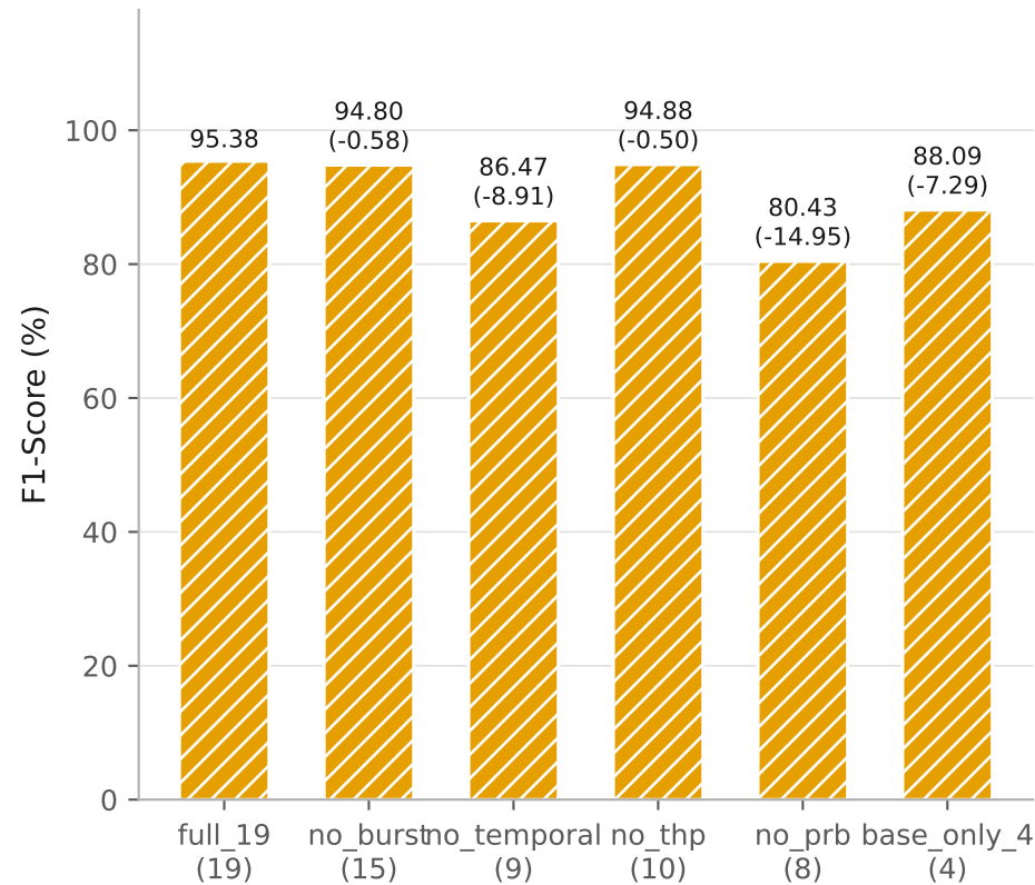
F1-Score
