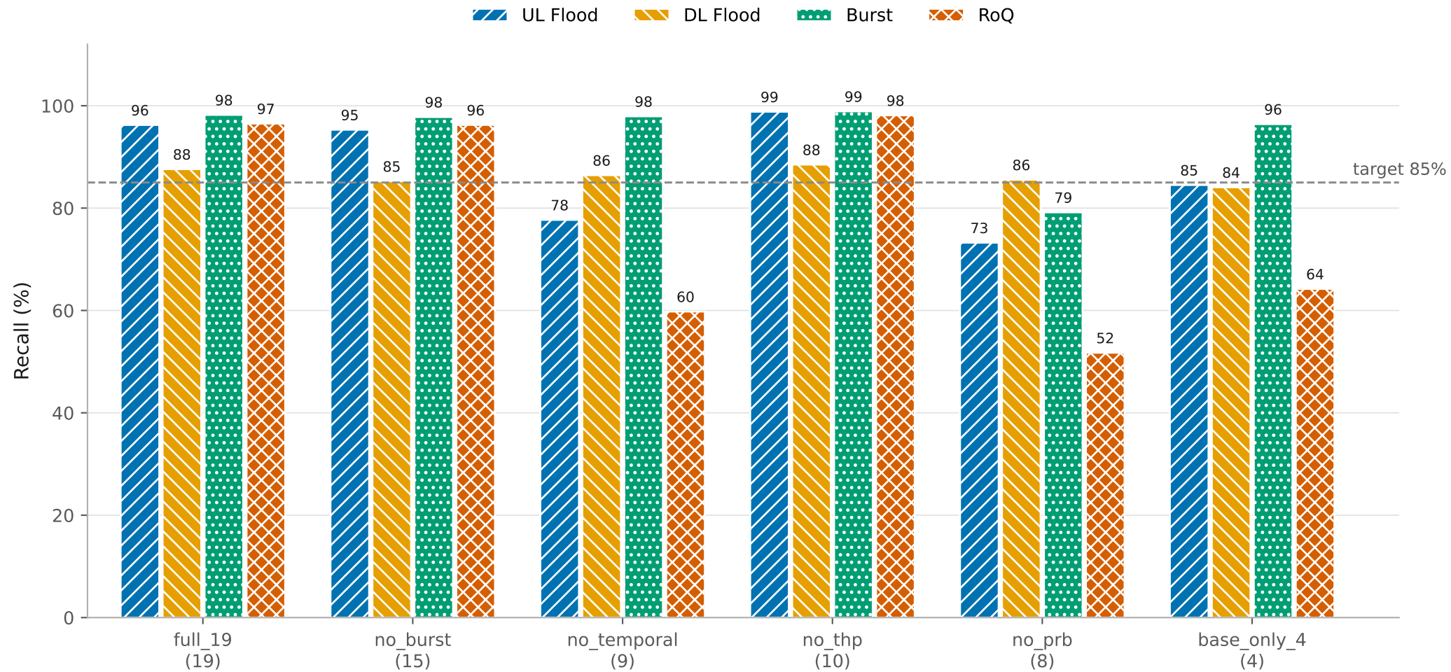
Per-Class Recall by Feature Configuration — GRU-AE, ML-Only (seed 42)
