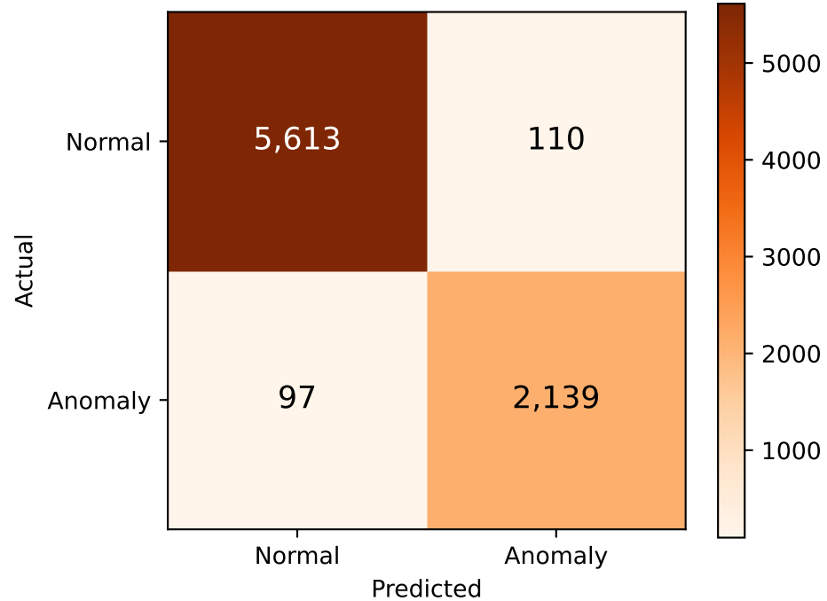
GRU-ONLY
