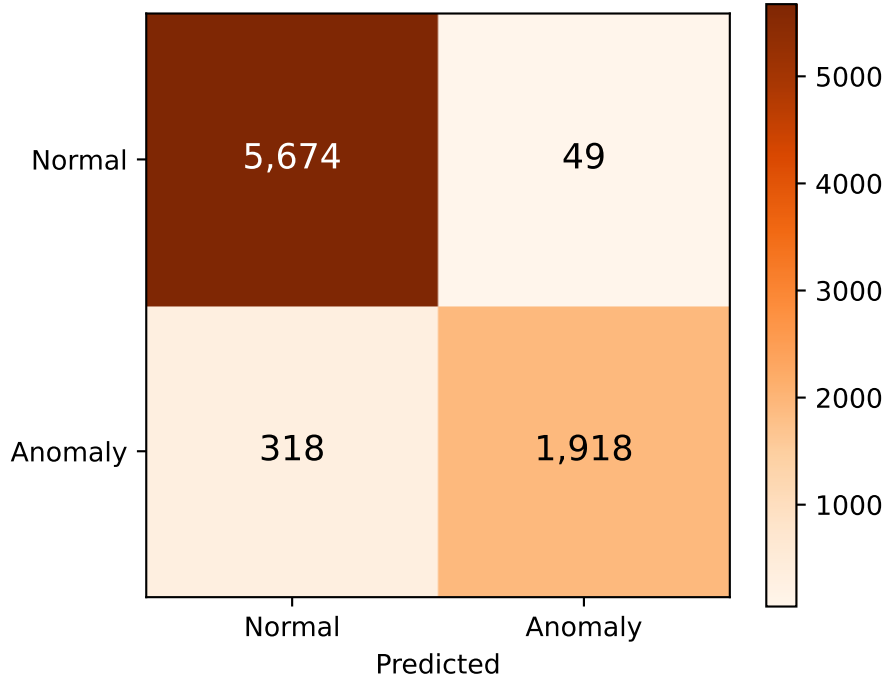
RULE-ONLY
