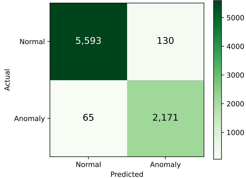
LSTM-ONLY
