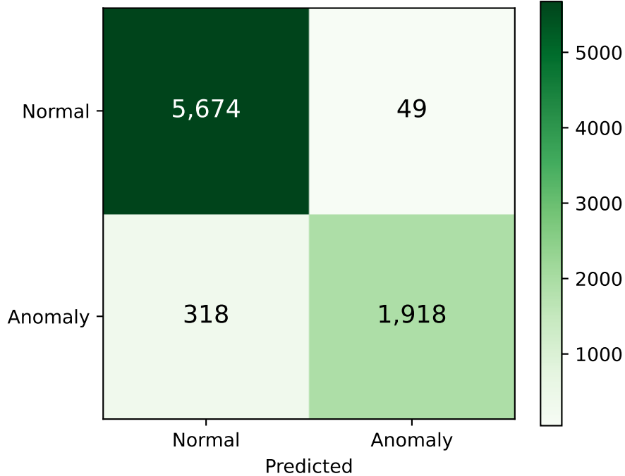
RULE-ONLY
