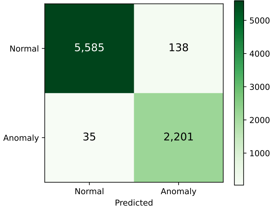
LSTM-HYBRID
