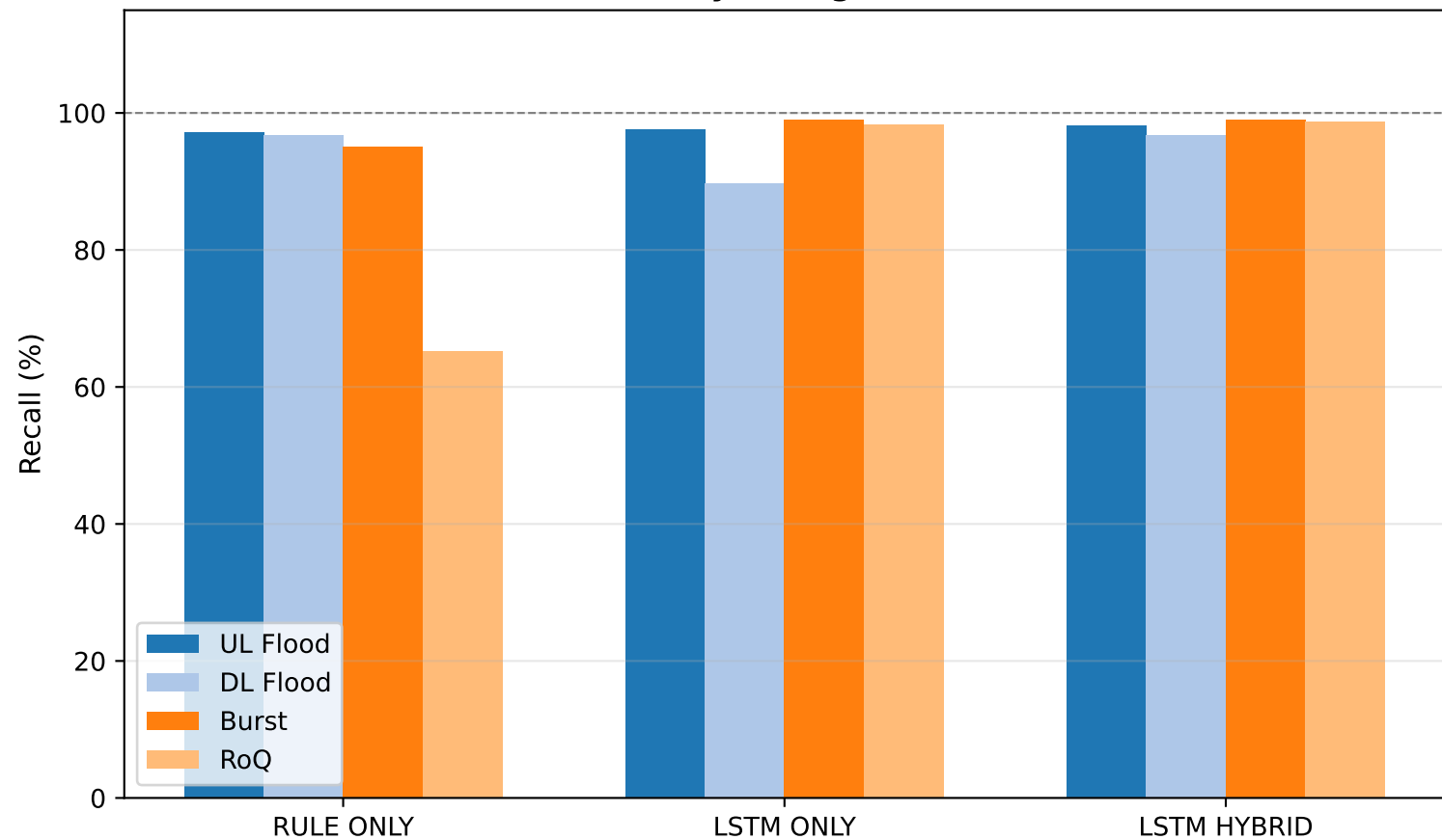
Per-Class Recall by Configuration (LSTM-AE)
