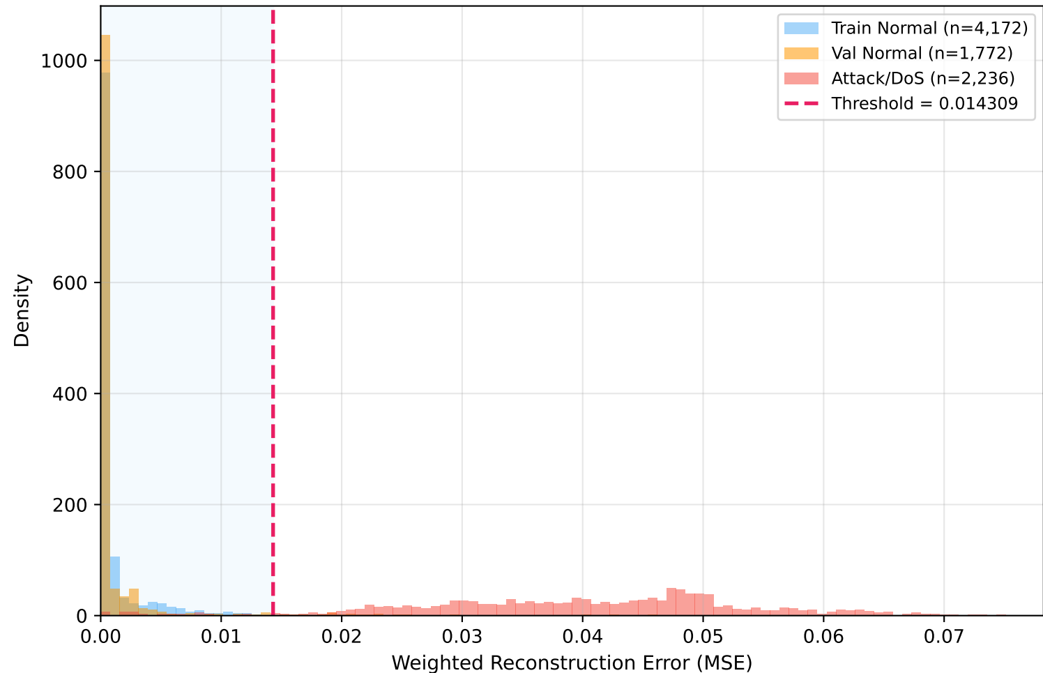
GRU-AE Reconstruction Error Distribution
