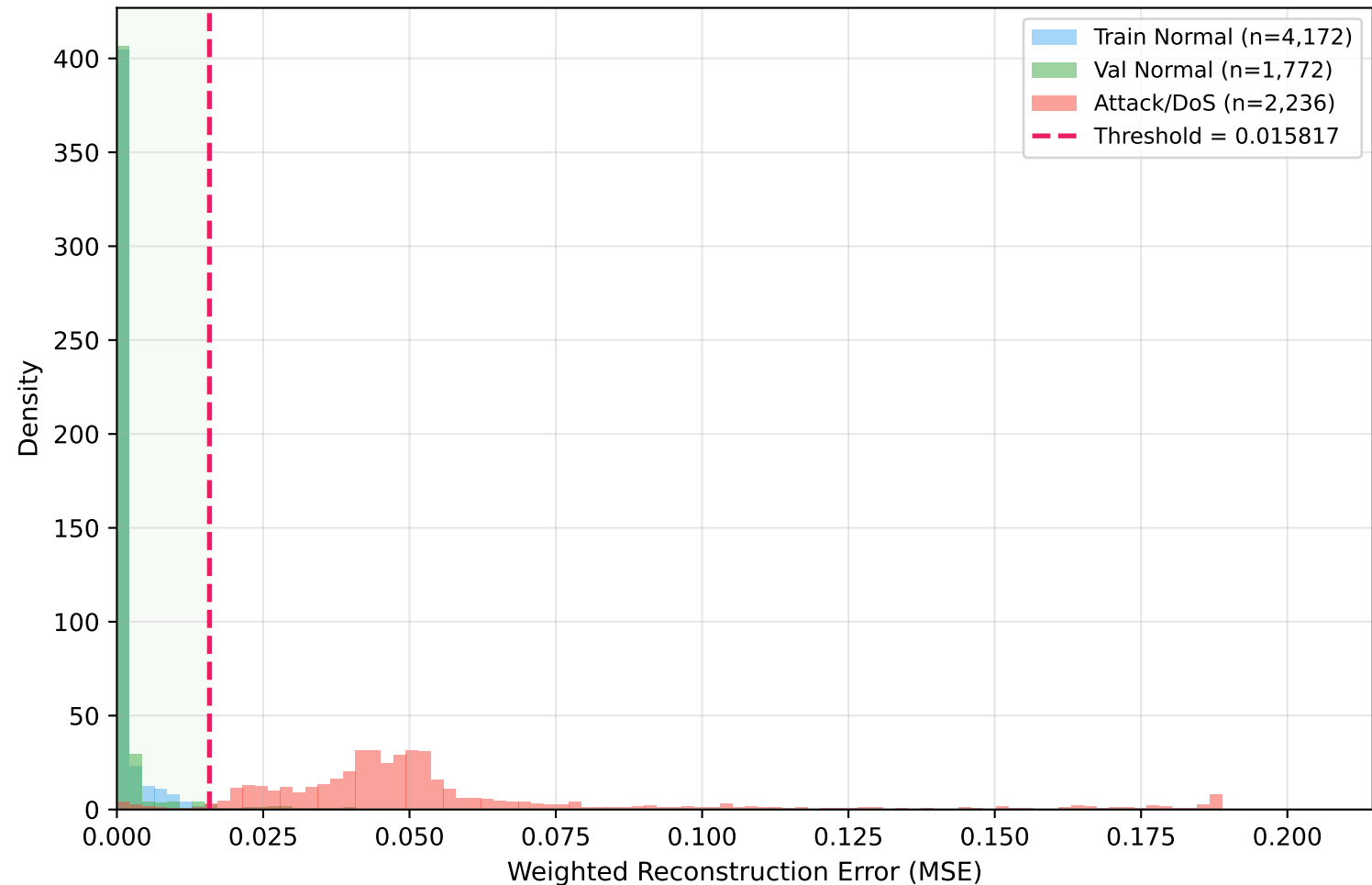
LSTM-AE Reconstruction Error Distribution
