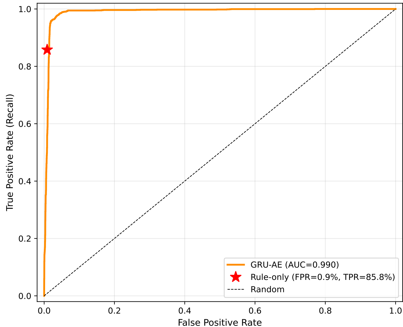
ROC Curve — GRU-AE
